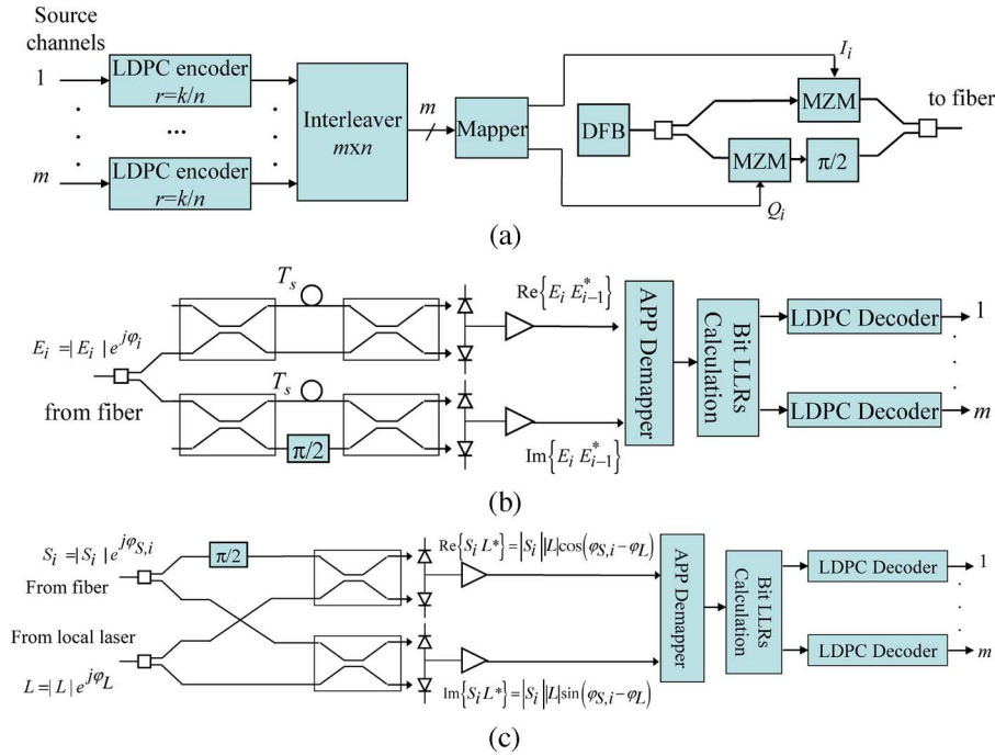
Fig. 1. BI-LDPC-CM scheme. (a) Transmitter architecture. (b) Direct detection as a reference case in accordance to [3]. (c) Coherent detection receiver architecture. T_s = 1/R_s , where R_s is the symbol rate.
