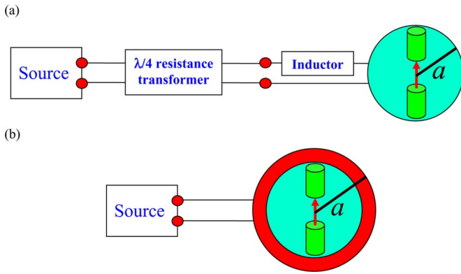
Fig. 1. (a) Traditional electrically small electric dipole antenna system having an inductive element to produce a total input reactance equal to zero, i.e., X_{\text{ind}} = X_{\text{ant}}^* so that X_{\text{input}} = 0 and a quarter-wavelength resistance transformer to match the input resistance to the source, and (b) the metamaterial-based EESA paradigm, i.e., the entire antenna system, including the radiating and matching elements, are electrically small defined by the smallest enclosing riansphere.
