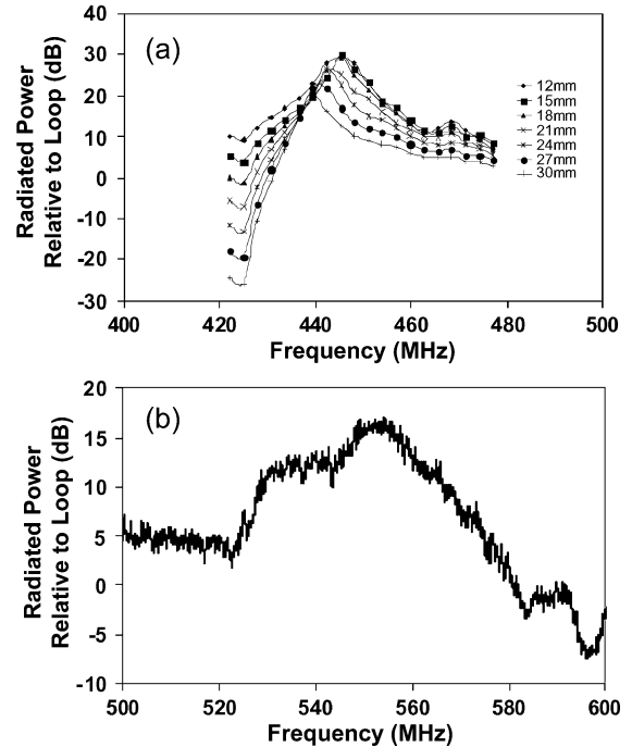
Fig. 3. (a) Simulated total radiated power of a hemispherical ESA with respect to the bare magnetic loop ( r = 0.9 cm) used to drive the antenna. (b) Measured total radiated power relative to the bare loop.
