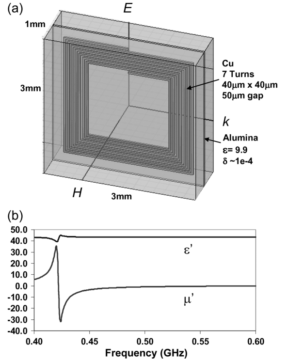
Fig. 2. Unit cell design showing (a) copper spirals on an alumina substrate and (b) retrieved \epsilon' and \mu' from the simulated scattering parameters.
