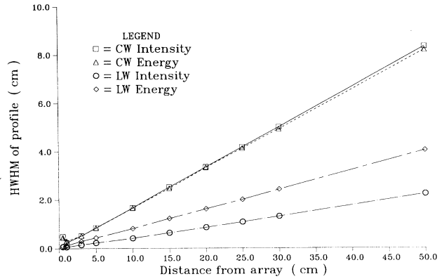
FIG. 6. Comparison of the expansion (half width at half maximum) along the line-of-sight direction of the radiated-field-energy and maximum intensity profiles of the beams generated by the LW and CW pulse-driven arrays.
