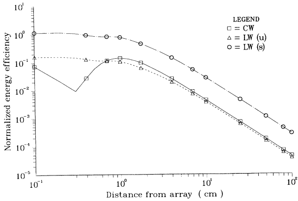
FIG. 4. Comparison of the decay of the radiated-field energy along the line-of-sight direction of the beams generated by the LW and CW pulse-driven arrays.
