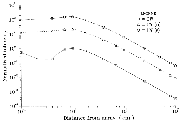
FIG. 5. Comparison of the decay of the maximum radiated-field intensities along the line-of-sight direction of the beams generated by the LW and CW pulse-driven arrays.
