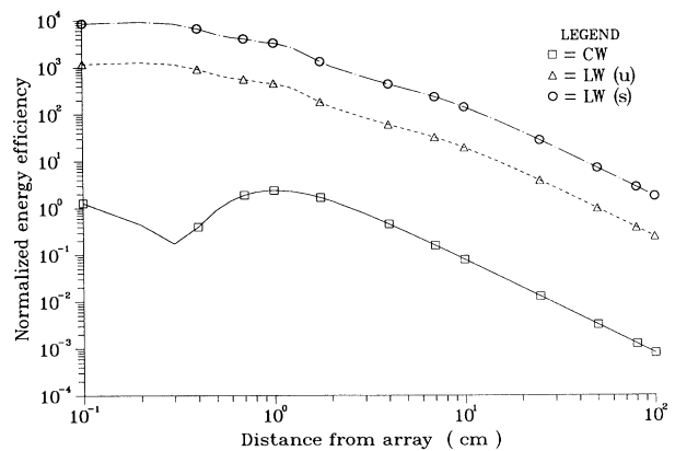
FIG. 7. Comparison of the decay of the measured-field energy along the line-of-sight direction of the beams generated by the LW and CW pulse-driven arrays.
