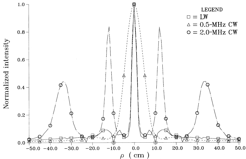
FIG. 9. Comparison of the normalized measured-field-intensity profiles at z = 30.0 cm of the beams generated by the LW and 0.5- and 2.0-MHz CW pulse-driven arrays.
