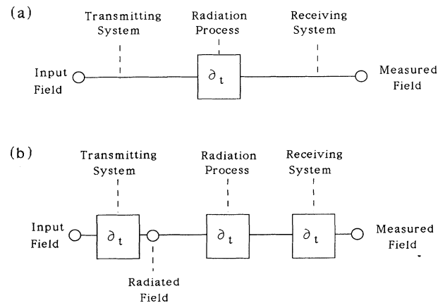
FIG. 2. The relationships between the input, radiated, and measured fields: (a) when k_{\max} l \gg 1 , and (b) when k_{\max} l \lesssim 1 .
