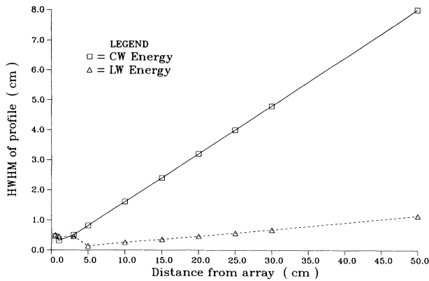
FIG. 8. Comparison of the expansion (half width at half maximum) along the line-of-sight direction of the measured-field-energy profiles of the beams generated by the LW and CW pulse-driven arrays.
